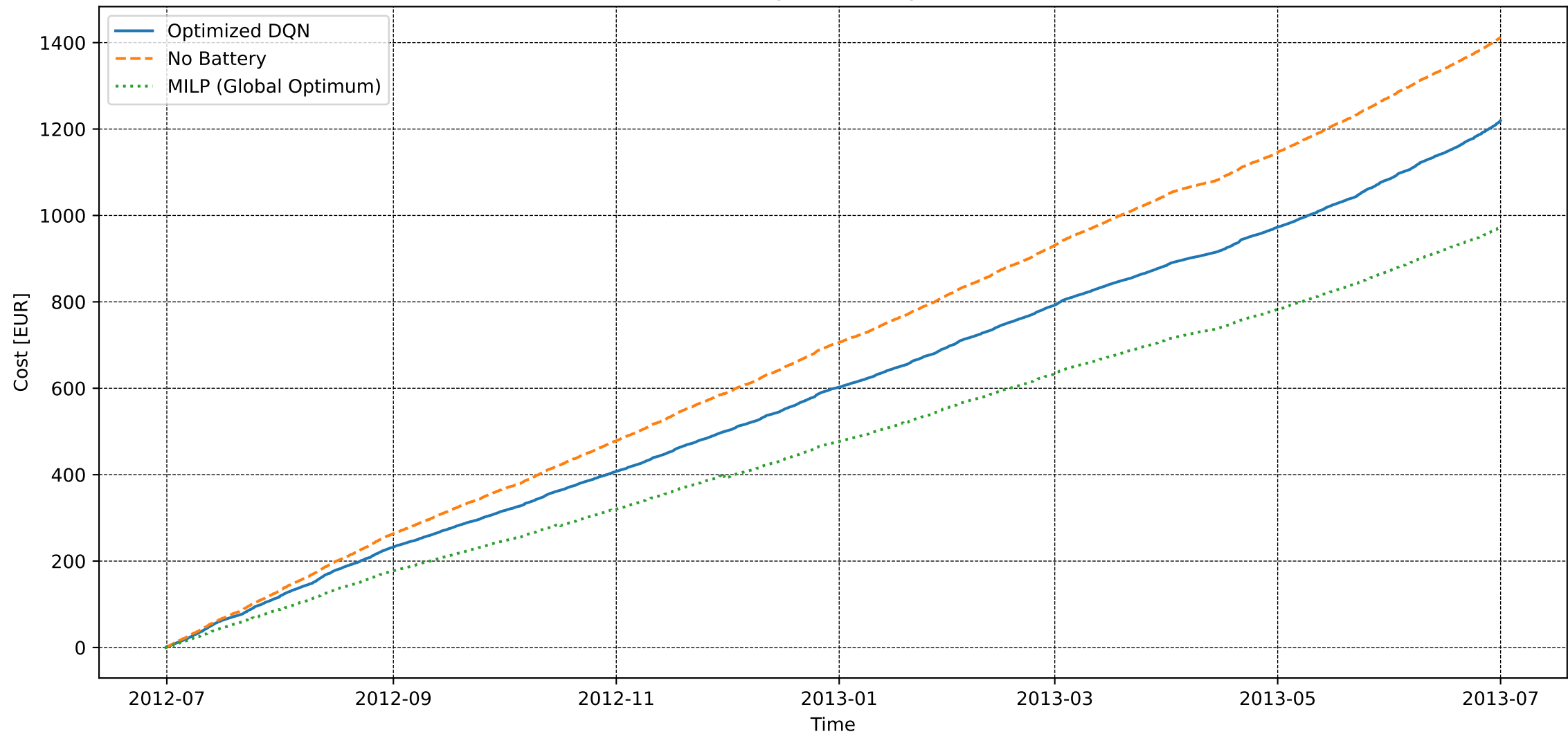
User 67 - Basic Training - Electricity Cost [DQN vs MILP]
